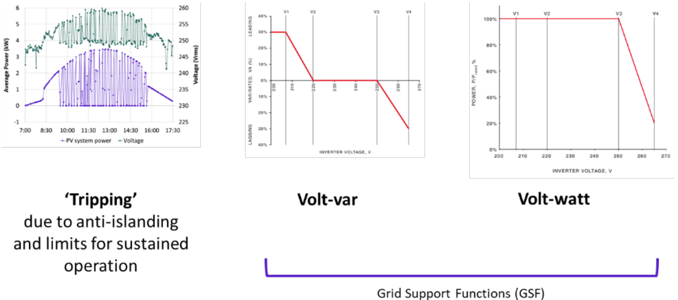
Figure 1 Potential causes of DER over-voltage curtailment
